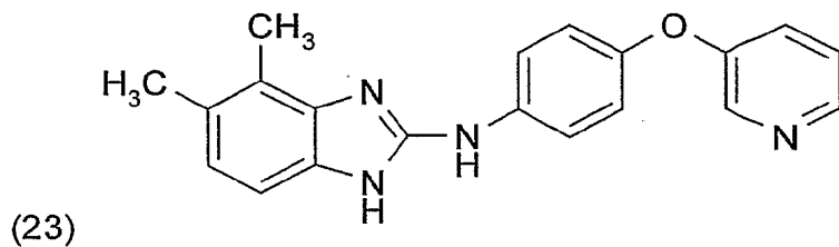
(4,5-Dimethyl-1H-benzimidazol-2-yl)-[4-(pyridin-3-yloxy)-phenyl]-amin
